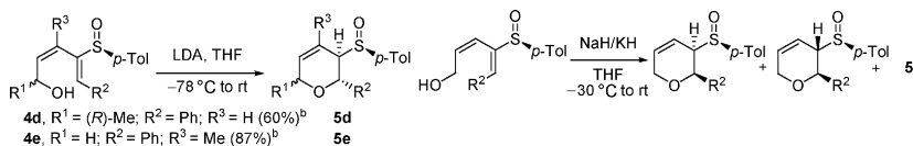
SCHEME 3 Synthesis of sulfinyl dihydropyrans.
