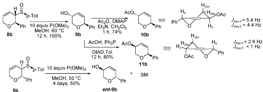
SCHEME 4 Structural assignments: sigmatropic rearrangements.
