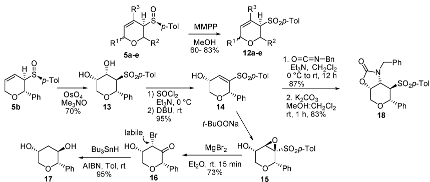
SCHEME 5 Synthetic applications.
