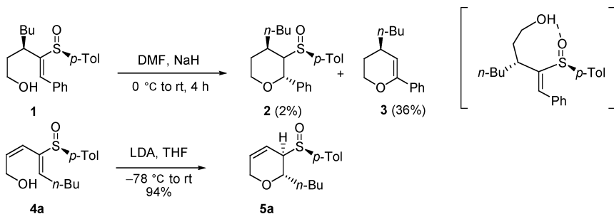
SCHEME 2 Base-promoted cyclization of hydroxy dienyl and vinyl sulfoxides.
