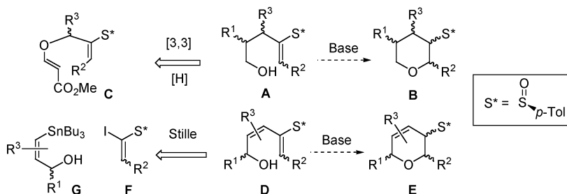
SCHEME 1 Proposed base-induced cyclization of hydroxy vinyl sulfoxides.
